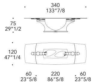
EXTENDABLE Square-round 220-340
