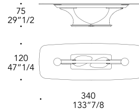
FIXED Square-round 340
