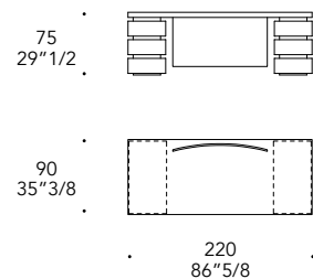
2 drawer units with front panel
